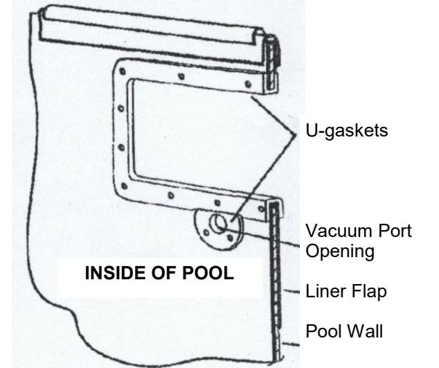
SECTION VIEW Stretch-in liner shown.
